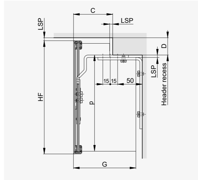
1.3 Straight cover.
